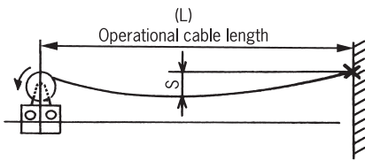
Horizontal stretch
