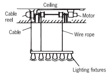
Stage lighting system
