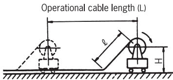
Horizontal retrieve
