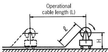
Horizontal retrieve
